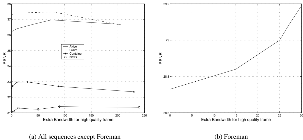
Figure 4: Plot of PSNR versus amount of high-quality for a jump update parameter of 50. Foreman has a separate figure because the extra bandwidth allocation for Foreman is distinctly different. This is the result of extra motion vector coding required for Foreman for the same quantization parameter values as compared to other sequences.
