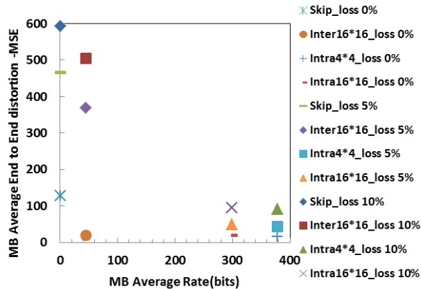
Figure 1: Average R-D operating points of various modes in different packet loss rates.
