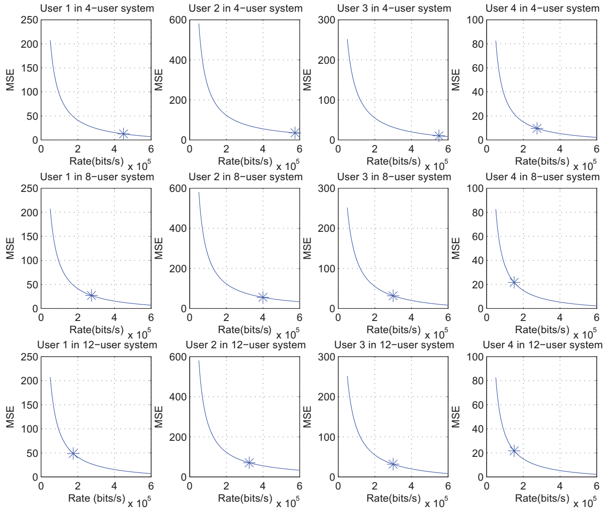
Fig. 7. Individual user's performance in systems with different number of users. Each column indicates the same user's RD relations in systems with four, eight and twelve users.
