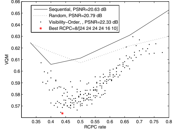
Fig. 5. VQM vs. R_{rpc} for both visibility-based and baseline algorithms optimized for the whole sequence, for systems with SNR = 8 dB, (N, M) = (32, 4) , f_{nd} = 10^{-4} . “MedMot” video is considered.
