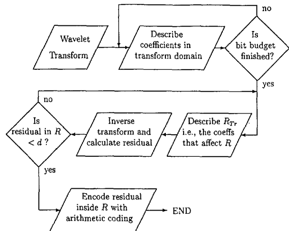
Fig. 8. Flow graph of the WA-algorithm.
