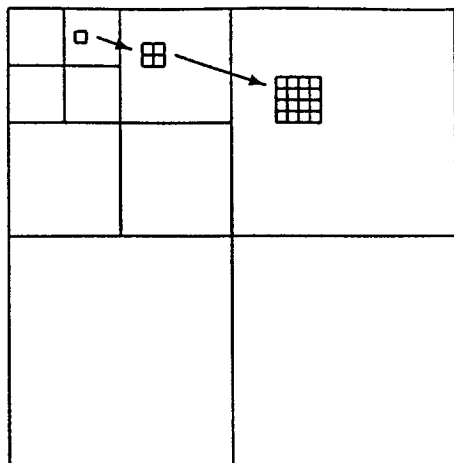
Fig. 4. Parent-child relationships in octave-band subbands.
